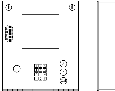
1837 Flush 12" W x 13.5" H x 2.5" D 305mm W x 343mm H x 63.5mm D
